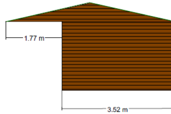
WEST ELEVATION
